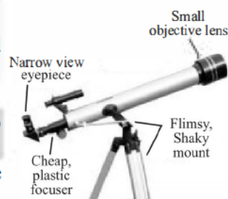
Fig: 13.25. Mechanical parts of a refracting telescope
